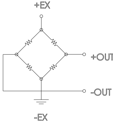
EQUIVALENT SCHEMATIC
